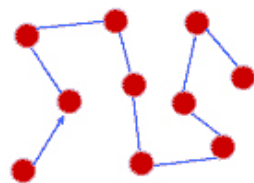
Brownian Movement of a Particle
