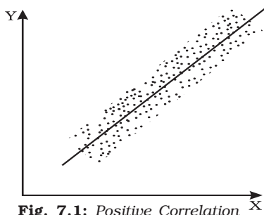
Fig. 7.1: Positive Correlation
