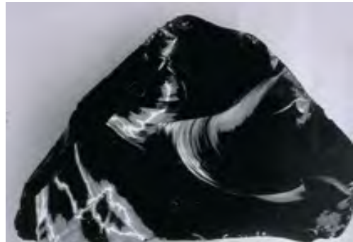
Fig 1.6: Obsidian
