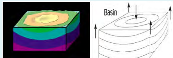
Fig. 4.21: Basin
