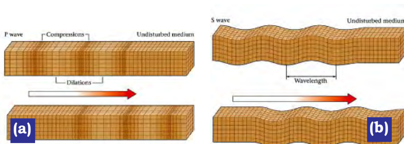
Fig. 7.8: (a) Primary waves and (b) Secondary waves
