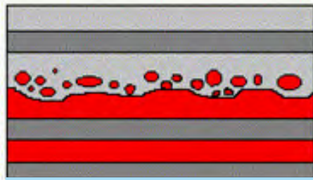
Fig 5.10: Clasts in an unconformity
