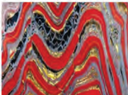
Fig.2.6: Banded iron formations
