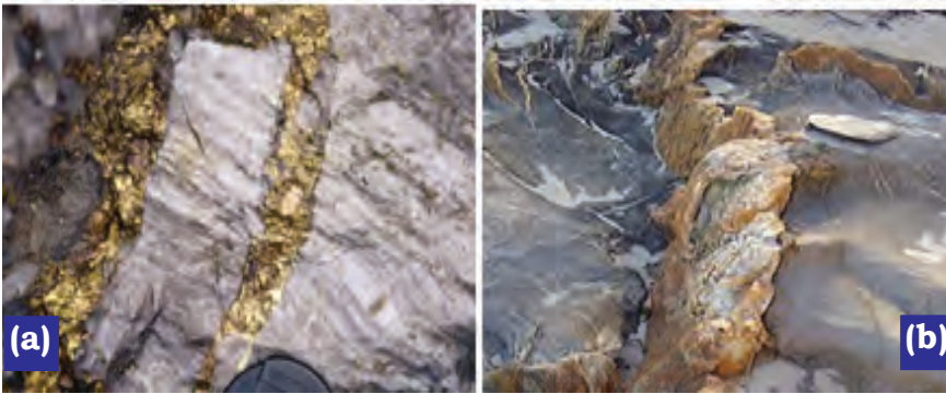
Fig. 2.5: Examples of vein type mineral deposits
