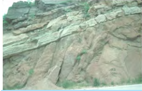
Fig. 4.36: Nonconformity
