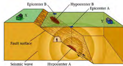
Fig. 7.3: Focus and epicenter of earthquakes
