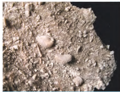
Fig.1.24: fossiliferous limestone
