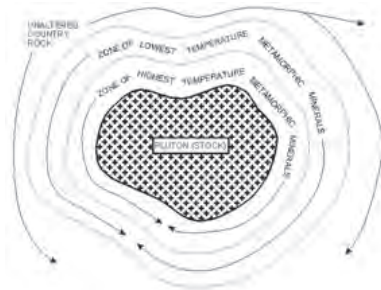
Fig. 1.26: Zones of contact metamorphism
