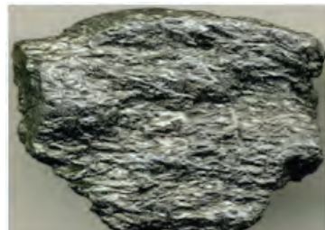
Fig. 1.29: Schist
