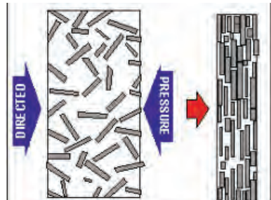
Fig.1.25: Diagram showing effect of pressure during metamorphism
