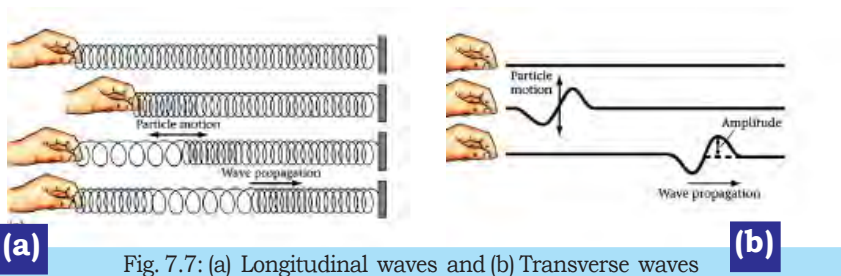
Fig. 7.7: (a) Longitudinal waves and (b) Transverse waves
