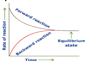
Attainment of equilibrium in a reversible reaction
